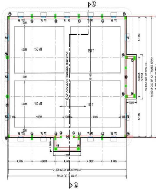
PLAN FOR 600 MT WH. BLDG.
