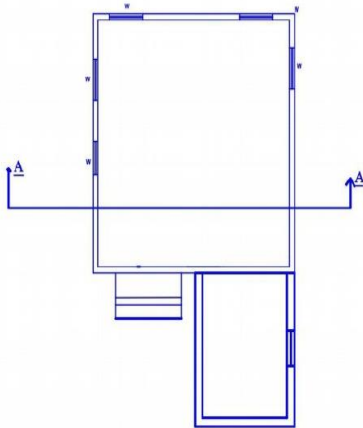
G.F. PLAN SCALE-1:100
